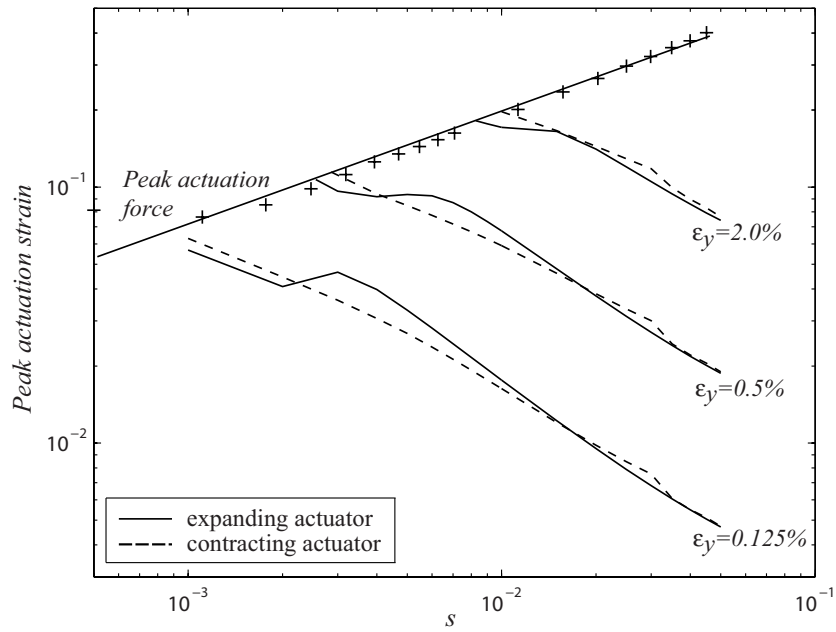
Figure 7: Peak actuation strain achievable for the flexible actuator before either the material yields, or a peak force is reached in the actuator.
