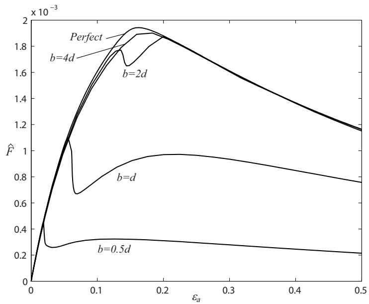
Figure 12: Actuation force versus actuation strain for kagome lattice models of s = 0.01 with a flexible actuator and rectangular bars. The in-plane dimension d is kept constant, and the out-of-plane dimension b varies. The ‘perfect’ result is included for comparison.
