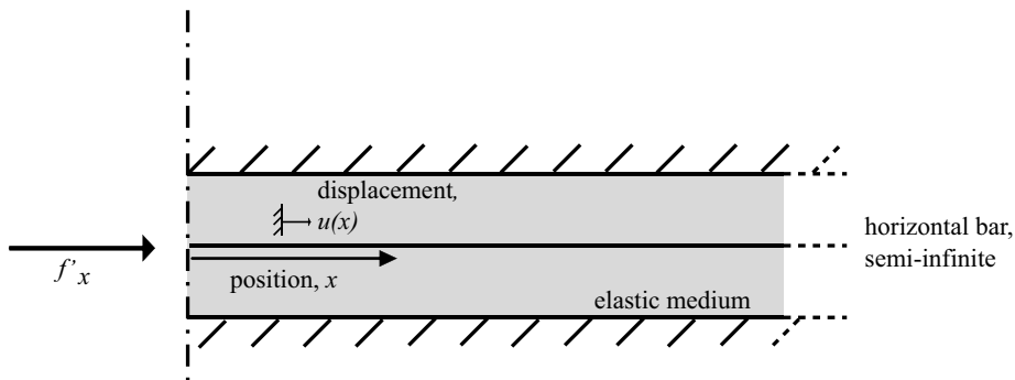
Figure 13: Smeared stiffness model, where a bar is suspended in an elastic material; adapted from Wicks & Guest (2004).
