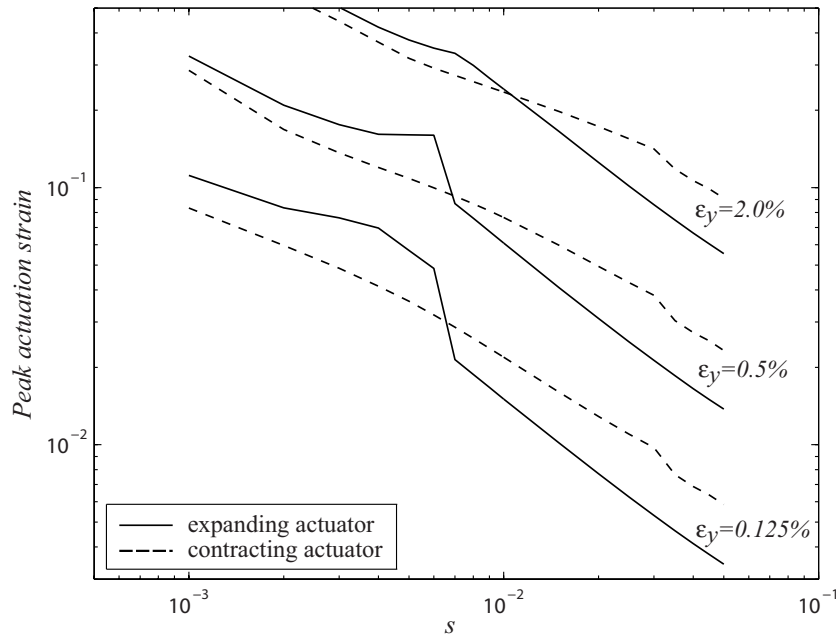
Figure 8: Peak actuation strain achievable for the stiff actuator before either the material yields, or a peak force is reached in the actuator.
