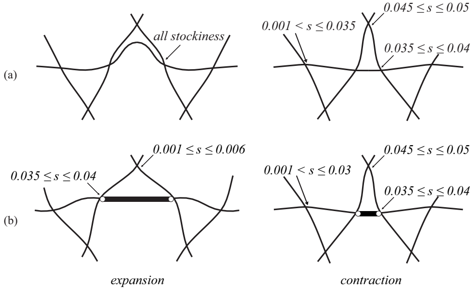
Figure 9: The position of the peak strain in the kagome lattice due to the actuation of a single bar, indicated by arrows, with a (a) flexible, and (b) stiff actuation.
