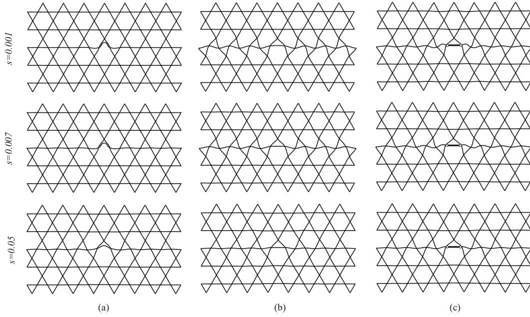
Figure 3: Deformed kagome lattices under positive actuation for \varepsilon_a = 0.5 and different values of bar stockiness: (a) non-linear actuation with a flexible actuator, (b) linear calculation and (c) non-linear actuation with a stiff actuator.
