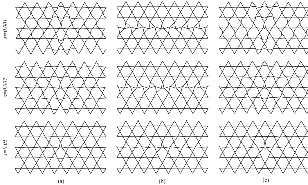
Figure 4: Deformed kagome lattices under negative actuation for \varepsilon_a = -0.5 and different values of bar stockiness: (a) non-linear actuation with a flexible actuator, (b) linear calculation and (c) non-linear actuation with a stiff actuator.
