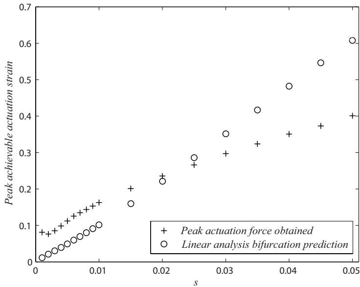
Figure 10: Comparison of limiting actuation strain at peak actuation force and buckling load.
