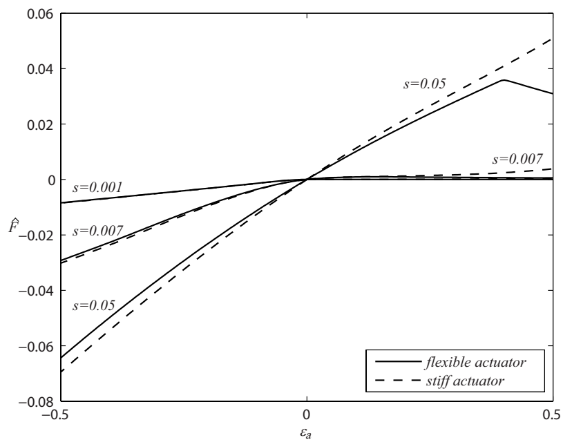
Figure 5: Non-dimensional actuation force calculated using geometrically non-linear models, for both flexible and stiff actuators, and s = 0.001 , s = 0.007 and s = 0.05 .
