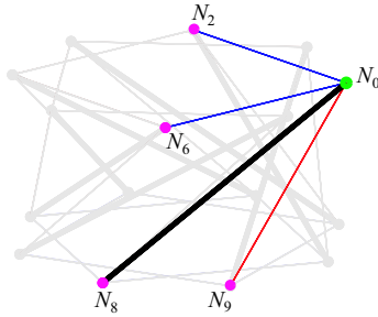
Fig. 2: All nodes connected to node 0, N_0 , of an example tensegrity structure with \mathbf{D}_8 symmetry. The horizontal cables are connected to nodes 2 and n-2=6 , the strut is connected to node n=8 , and the ‘vertical’ cable is connected to node n+1=9 . This structure is denoted \mathbf{D}_8^{2,1} .
